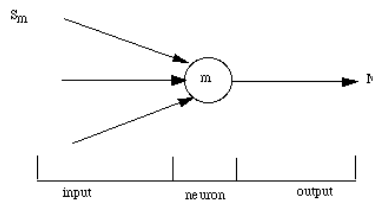
Figure 11. Simple neural element as basic component at the neural network level.
