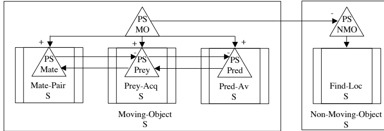
Figure 3. Rana Computatrix ethogram: Mating, Prey Acquisition and Predator Avoidance schemas (moving and non-moving objects) [8]. The diagram shows feedback between perceptual schemas (triangles) and regular schemas (rectangles). Note the hierarchical schema organization. (Acronyms are as follows: PS - Perceptual Schema, MO - Moving Object, NMO - Non-Moving Object, S -Schemas.)
