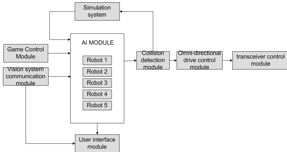
Fig. 3. Artificial Intelligence System Architecture.
