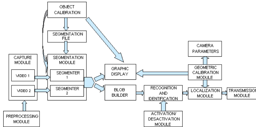
Fig. 2. Vision System Architecture.
