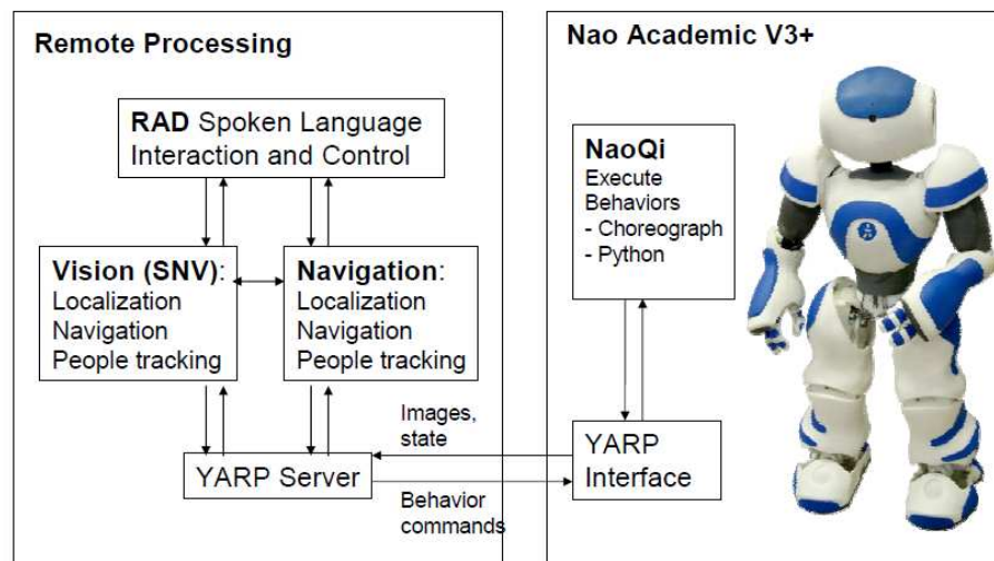
Fig. 5. Integrated system architecture overview. Running local on the Nao is the NaoQi system and the Urbi server.
