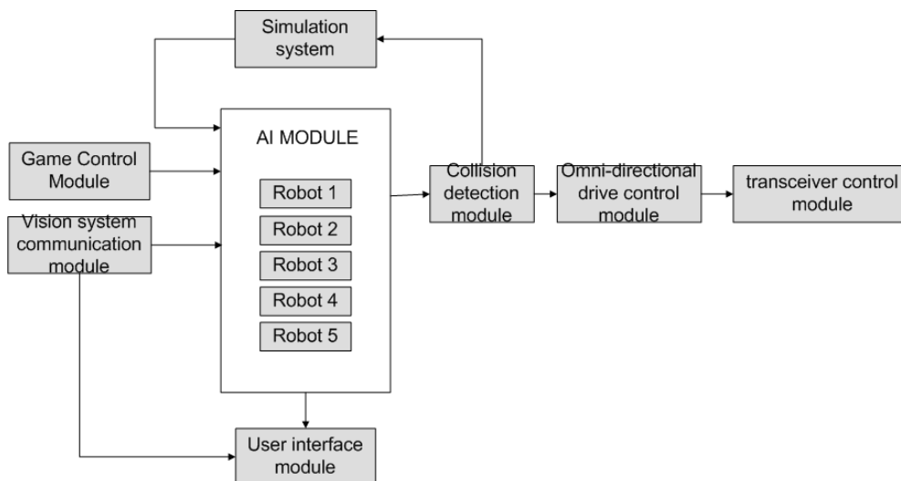
Figure 5. Artificial Intelligence System Architecture consisting primarily of the following modules: Game Control, Vision Communication, User Interface, Simulation, Collision Detection, Omni-directional drive control and Transceiver Control.
