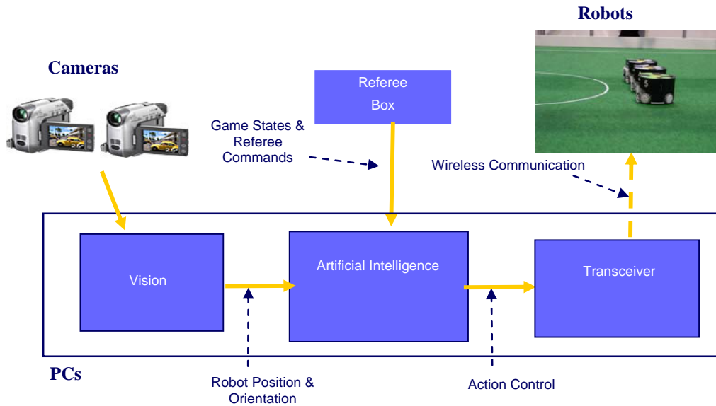
Figure 3. RoboCup Small-Size league block diagram. Visual input from cameras mounted on top of the field are processed by the Vision module to provide the AI module with robot positions and orientations. The AI module sends action command to the robots via a transceiver.
