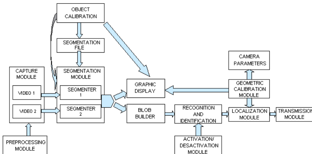
Figure 4. Vision System Architecture consisting primarily of the following modules: Capture, Segmentation, Calibration, Recognition and Identification, Activation and Deactivation, Localization and Transmission.
