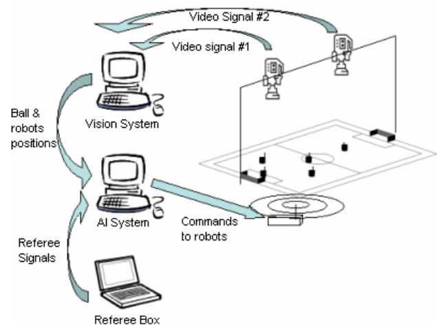
Figure 1. System configuration of the Small-Size League. Aerial cameras send video signals to a computer processing the vision system that in turns sends its output to an AI system responsible for remote robot control.
