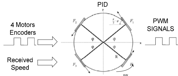
Figure 9. Motor control using Pulse Width Modulation (PWM) and Proportional-Integral-Derivative controller (PID).
