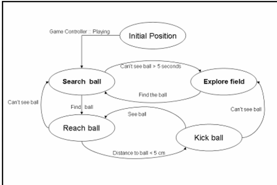
Fig. 4. Basic Individual Attacker State Machine.
